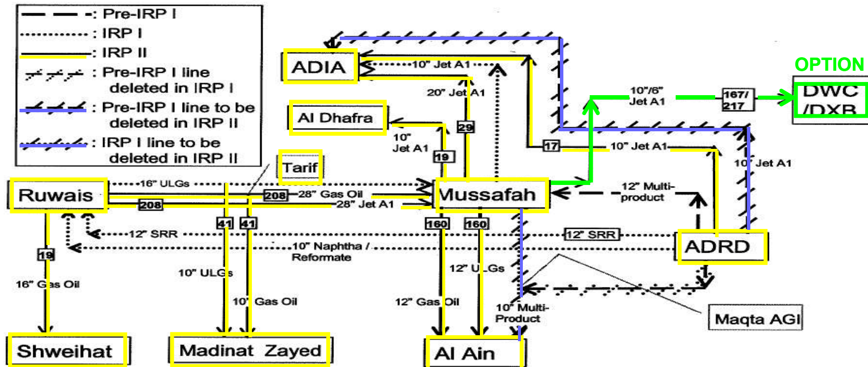
Figure 1: Simplified Block Diagram of Facilities
